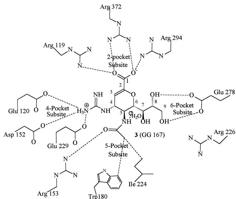
Figure 1. Cartoon showing the interactions of 3 (GG167) in the neuraminidase binding site (N9 numbering). Note that Tyr 406 lies under 3 and is not shown.
