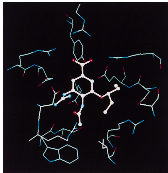
Figure 4. X-ray crystal structure of the binding site region for the complex formed between benzoic acid 11 and N9 neuraminidase.
