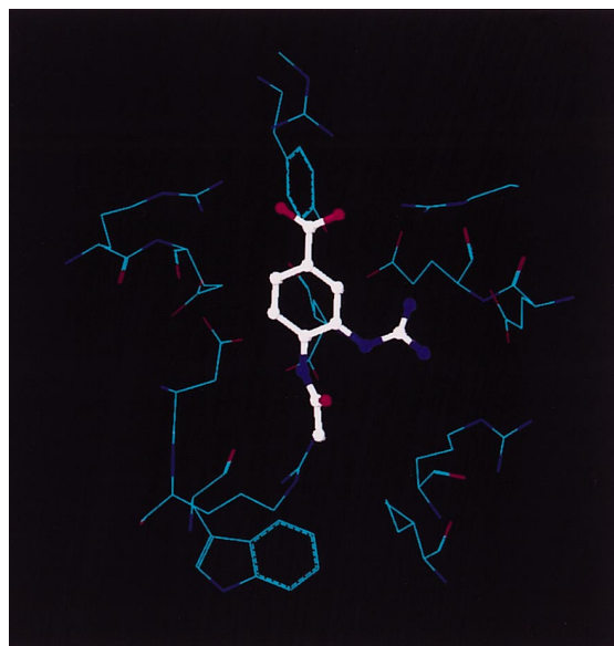
Figure 2. X-ray crystal structure of the binding site region for the complex formed between BANA 113 and N9 neuraminidase.
