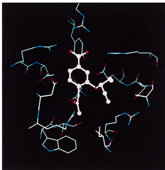
Figure 3. X-ray crystal structure of the binding site region for the complex formed between benzoic acid 8 and N9 neuraminidase.
